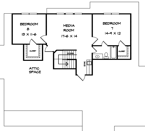
THIRD LEVEL FLOOR PLAN
