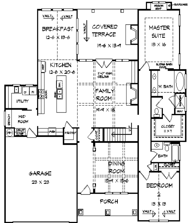
WIDTH - 58'-6" DEPTH - 60'-0" FIRST FLOOR PLAN
