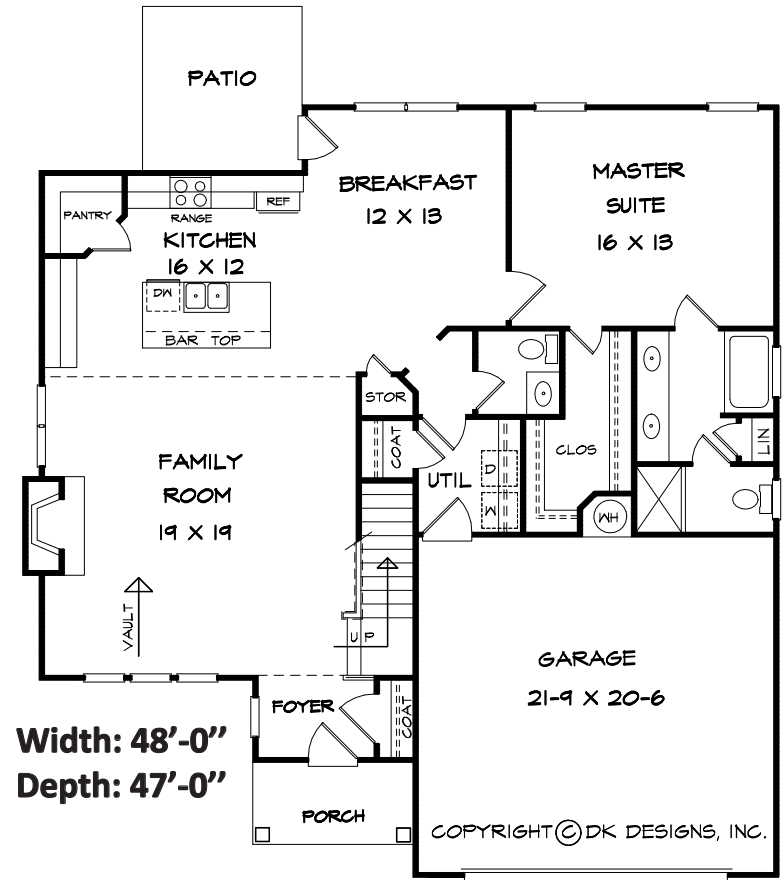
FIRST FLOOR PLAN A
