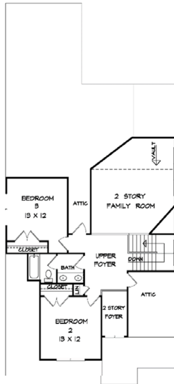
UPPER LEVEL FLOOR PLAN
