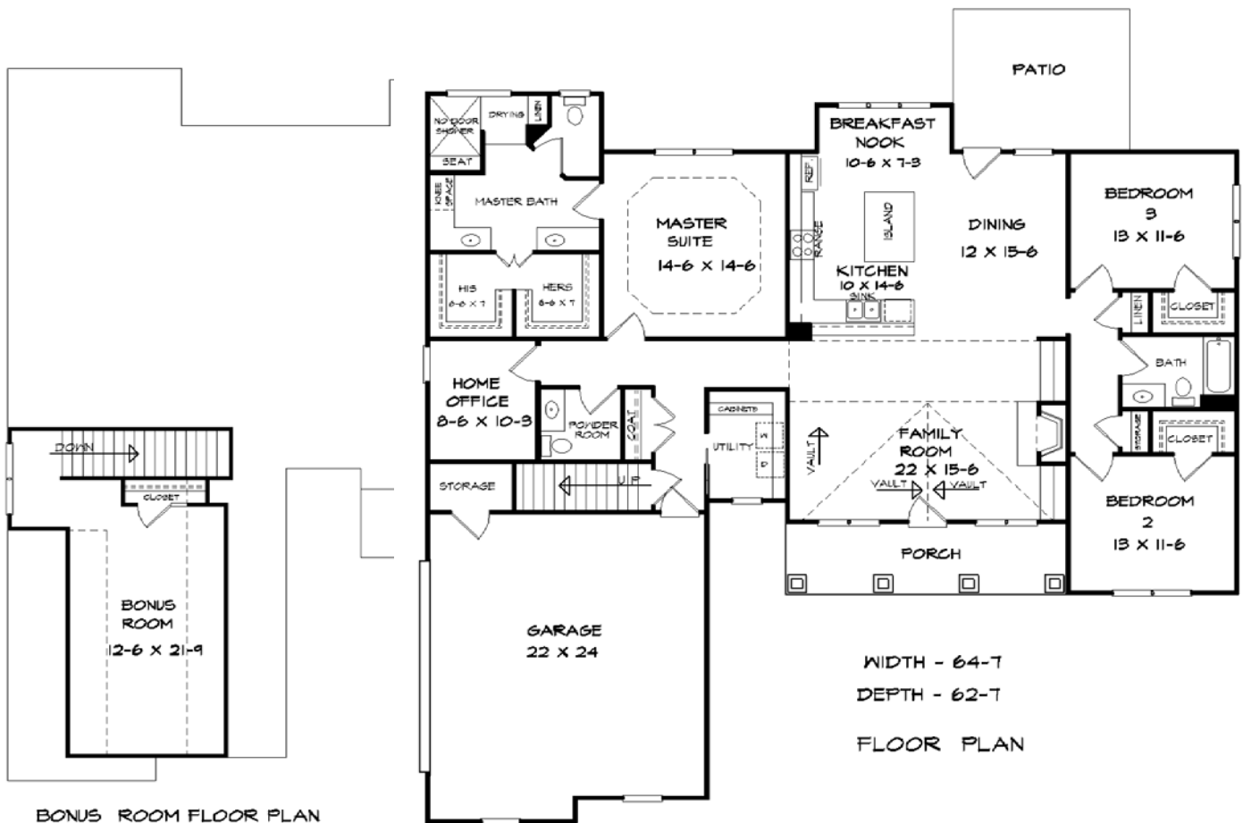
BONUS ROOM FLOOR PLAN BONUS ROOM ADDS - 360 SQ. FT.
