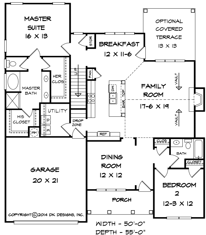
MAIN LEVEL FLOOR PLAN - A
