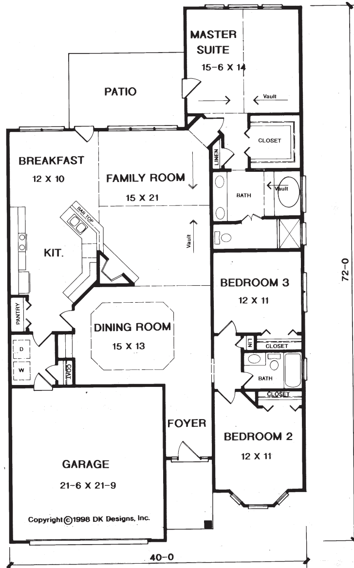
FLOOR PLAN
