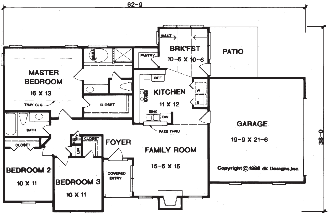
FLOOR PLAN
